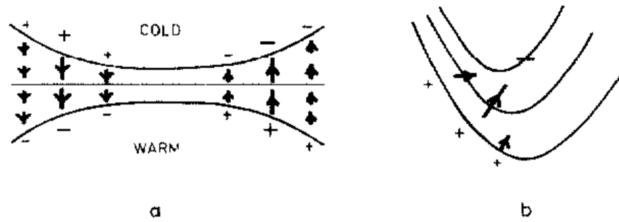
Figure 3. Two standard synoptic situations. (a) The height contours for a jet entrance and exit. (b) Temperature contours in a diffluent trough. Horizontal shears in the geostrophic velocity field are assumed to be dominated by the thermal wind contribution.
